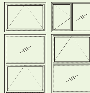
TOP HUNG Windows
