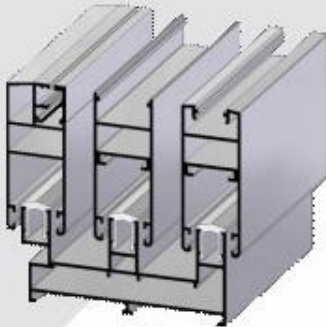
THREE TRACK WITH FLY SCREEN SHUTTER
